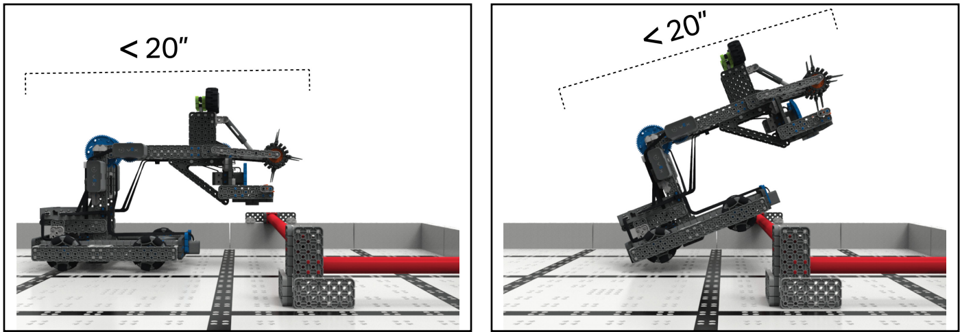
Figure 19: Examples of how a Robot should be measured horizontally.
